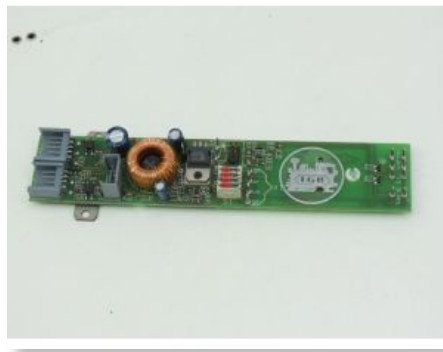
LGB 28001/ 28002 Platine
