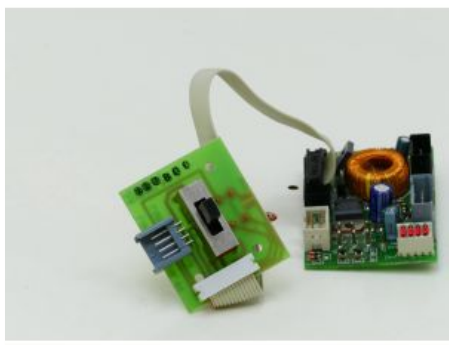
LGB 20802 Platine
